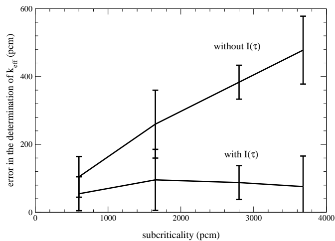
FIG. A.5 – Absolute errors in the determination of k_{\text{eff}}^P , function of 1 - k_{\text{eff}}^P with the two methods (with and without the importance weighting), and for the 4 different subcriticalities considered. The error bars show the statistical error
