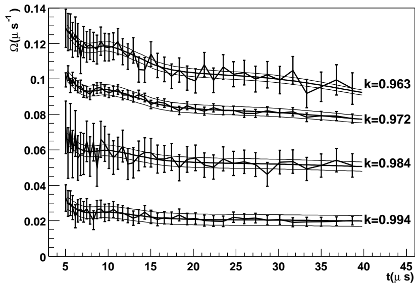
FIG. A.4 – \Omega_{k_{\text{eff}}^P}(t) fits for 4 reactors of different k_{\text{eff}}^P , after weighting P(\tau) by the importance
