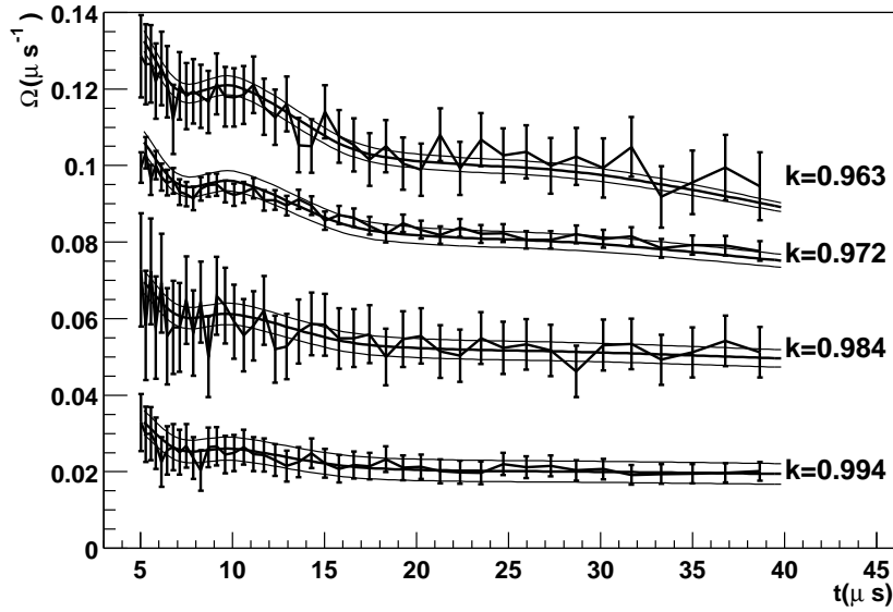
FIG. A.3 – \Omega_{k_{\text{eff}}^{\text{p}}}(t) fits for 4 reactors of different k_{\text{eff}}^{\text{p}} . The polygonal lines with error bars show the “real” decreases while the smooth curves show the fit results, \pm 100 pcm
