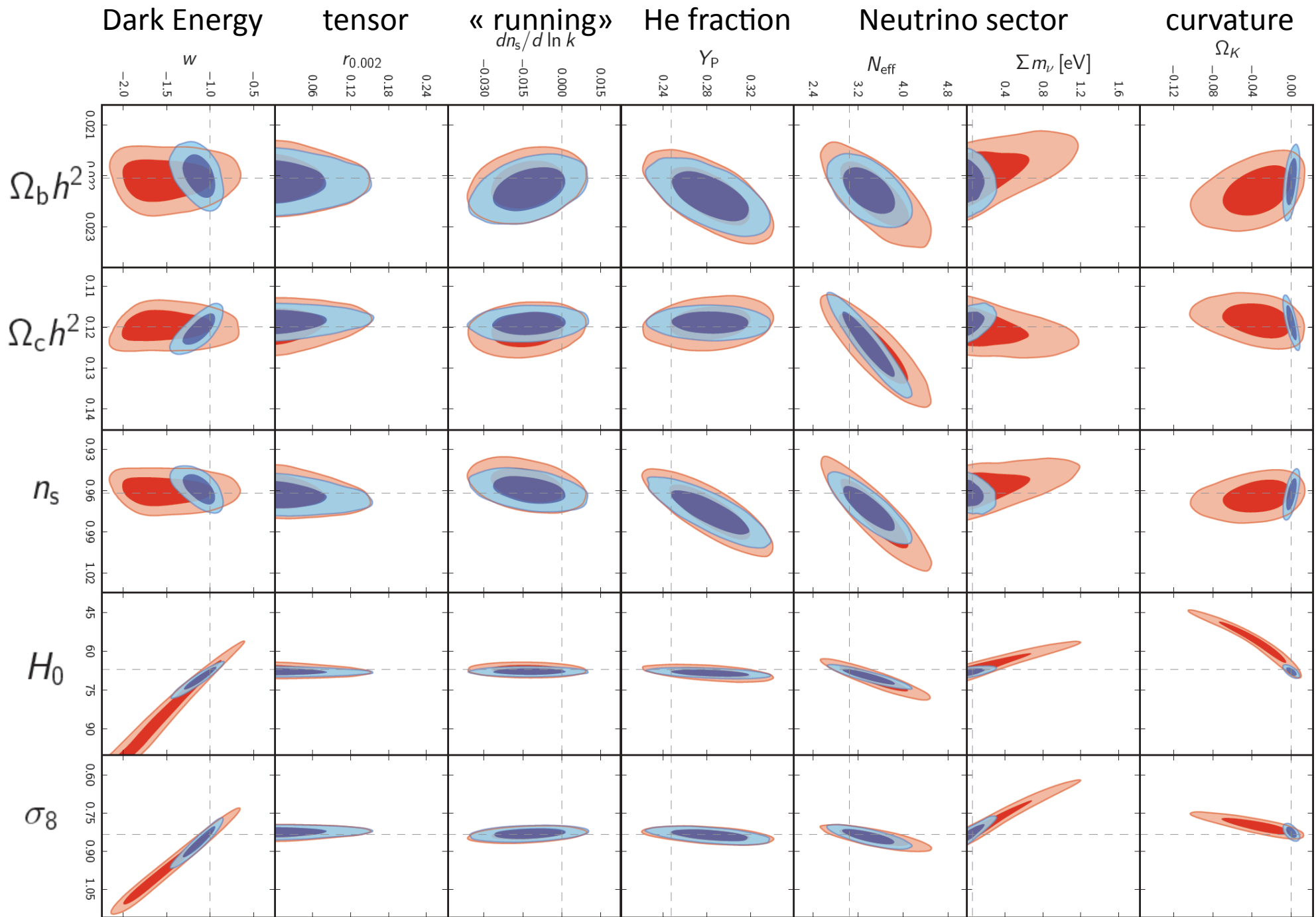
Planck 2013 results. XVI. Cosmological parameters ArXiv:1303.5076, Fig. 21
