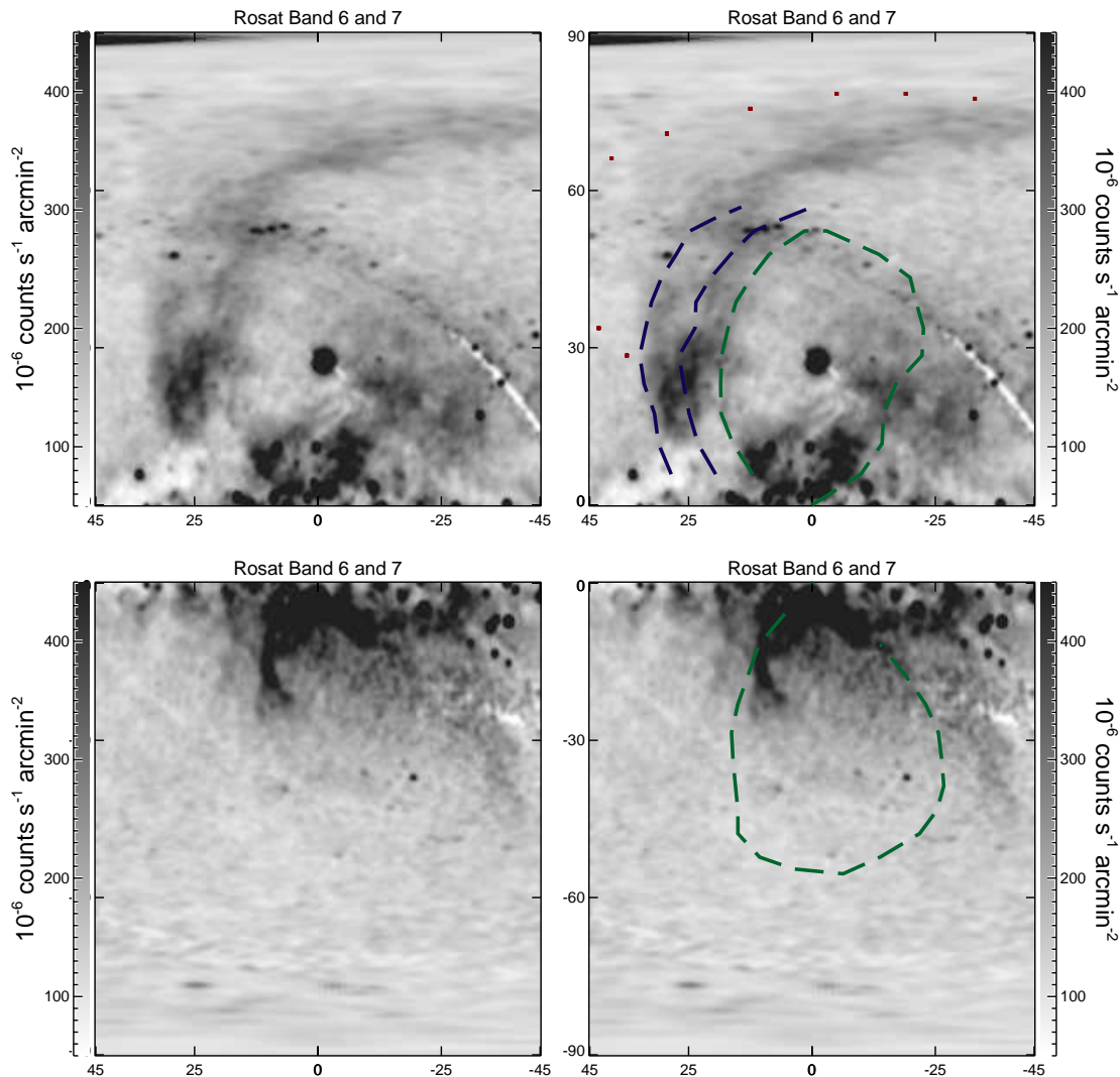
FIG. 19.— Top left: The ROSAT X-ray haze features compared with the Fermi bubbles' morphology. Top row: The X-ray features of ROSAT band 6 and 7 in the north sky towards to the GC ( left panel ) compared with Fermi north bubble overplotted with green dashed line, northern arc feature in blue dashed line, and Loop I feature in red dotted line ( right panel ). Bottom row: Same as top row but for the south bubble features.
