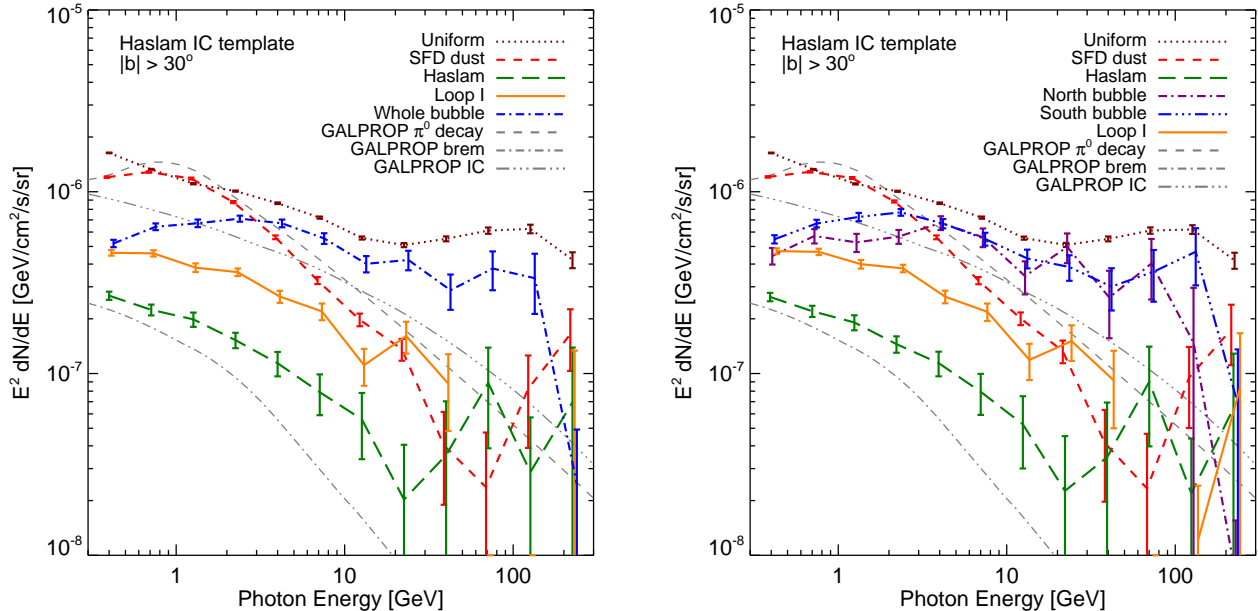
FIG. 17.— Same as Figure 12, but using the Haslam 408 MHz map instead of the simple disk model as the IC template. The Haslam map contains a bright feature associated with Loop I (see Figure 18) and is dominated by synchrotron emission from softer electron CRs, of energies around 1 GeV; it is not an ideal tracer of IC emission which depends on both electron and ISRF distribution. The resulting best-fit spectrum for the bubble template remains harder than the other components, but with enhanced lower energy ( \lesssim 2 GeV) correlation coefficients compared to Figure 12 and Figure 14. The right panel is the same as the left panel, but with the bubble template divided into north and south bubbles (see §3.2.2 for more discussion). As in Figure 12, the correlation spectra have been normalized to a reference region; see §3.2.2 for details, and Table 2 for a summary of the normalization factors.
