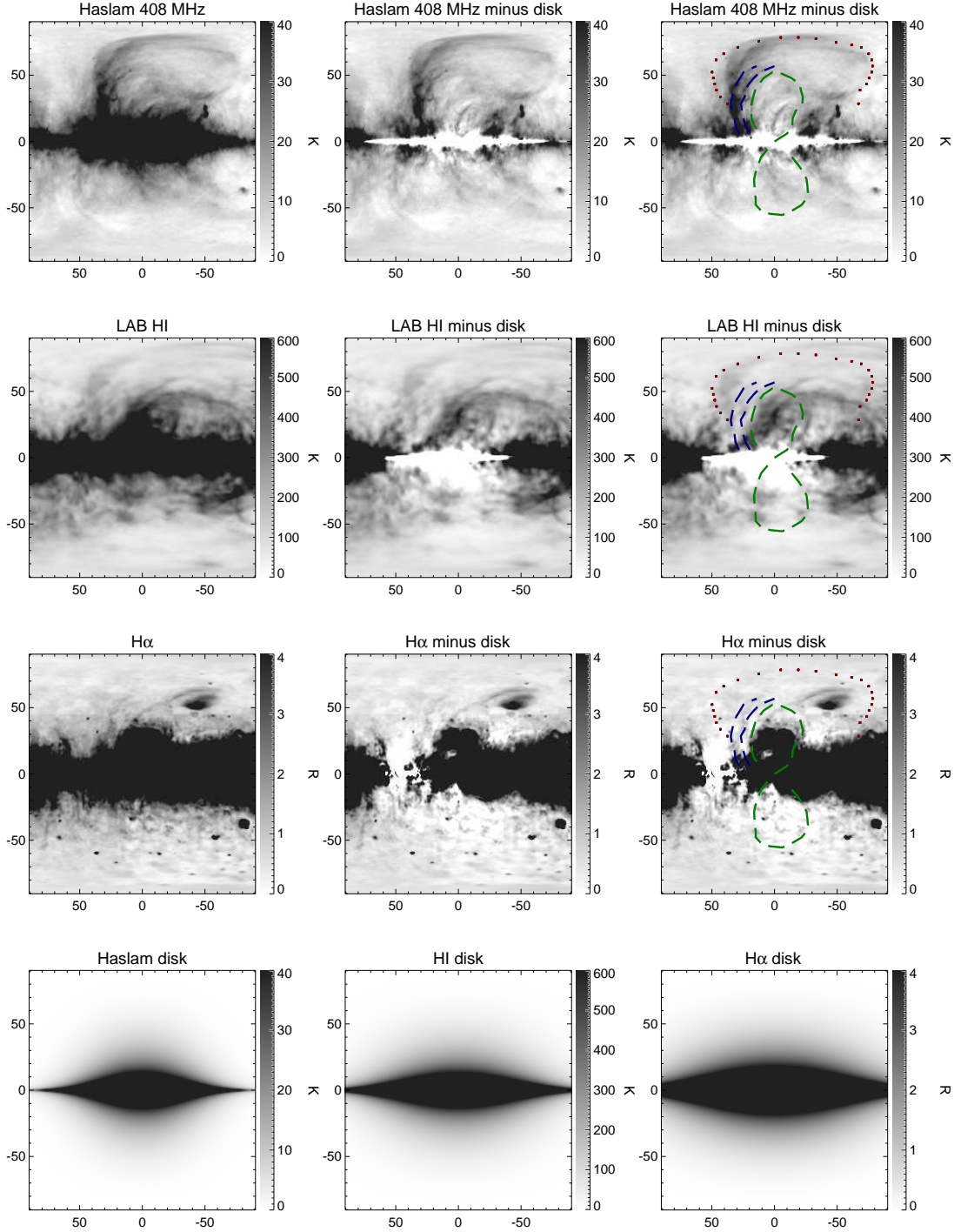
FIG. 26.— Fermi bubble features in other maps. Top row : The left panel shows the half sky Haslam 408 MHz map (Haslam et al. 1982) with -90^\circ < \ell < 90^\circ , the middle panel subtracts a simple geometric disk template (shown in the bottom left panel) to better reveal the structures deeper into the Galactic plane. The right panel is the same as the middle panel but overlaid with the Fermi bubbles, the northern arc , and the Loop I features identified from the 1 – 5 GeV Fermi gamma-ray map (see Figure 4). The Loop I feature ( red dotted line ) align with the extended diffuse features in the Haslam 408 MHz synchrotron map (known as North Polar Spur ). The inner and outer edges of the northern arc ( dashed blue lines ) overlap with two arcs in the Haslam synchrotron map. However, the Fermi bubbles have no apparent counterparts in this map. Second row : The same as the top row , but for the Leiden/Argentine/Bonn (LAB) Survey of Galactic HI (Kalberla et al. 2005). The middle panel subtracts a simple disk template shown in the bottom middle panel to better reveal structures towards the GC. No apparent features have been identified that correlate with the Fermi bubbles and other features in 1 – 5 GeV Fermi map (there may be some faint filaments morphologically tracing the gamma-ray features). Third row : The same as the top row but for the H \alpha map (Finkbeiner 2003). The middle panel subtracts a simple disk template shown in the bottom right panel to reveal more structures in the inner Galaxy. No corresponding features have been identified morphologically similar to the structures in the 1 – 5 GeV Fermi gamma-ray maps (color line in the right panel).
