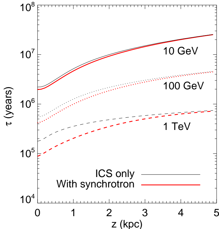
FIG. 28.— The cooling time for electron CRs as a function of energy and height above the Galactic plane, for r = 0 . Thin black lines : Synchrotron losses are neglected; equivalently, the B-field is assumed to be negligible everywhere. Thick red lines : The cooling time calculation includes synchrotron losses in a magnetic field given by |B| = 30e^{-z/2\text{kpc}}\mu\text{G} . We use the standard radiation field model from GALPROP version 50p, and define the cooling time \tau = 1/(d \ln E/dt) .
