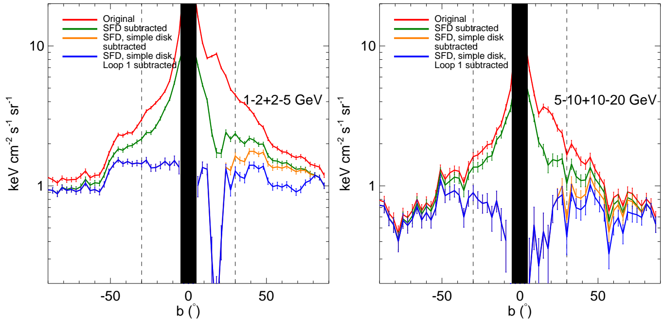
FIG. 9.— Intensity averaged over the central 20 degrees in longitude, as a function of latitude, for ( left ) the averaged 1–2 and 2–5 GeV maps, and ( right ) the averaged 5–10 and 10–20 GeV maps. We construct great circle arcs perpendicular to the l = 0 great circle, extending 10^\circ in each direction (east and west), and average the emission over each such arc; the “ b ” label corresponding to each arc, and the x -axis of the plot, refers to the value of b at l = 0 . Different lines show the results at different stages of the template subtraction process. The large oversubtraction at b \sim 15^\circ in the north, especially pronounced in the low-energy data, is associated with a bright feature in the SFD dust map.
